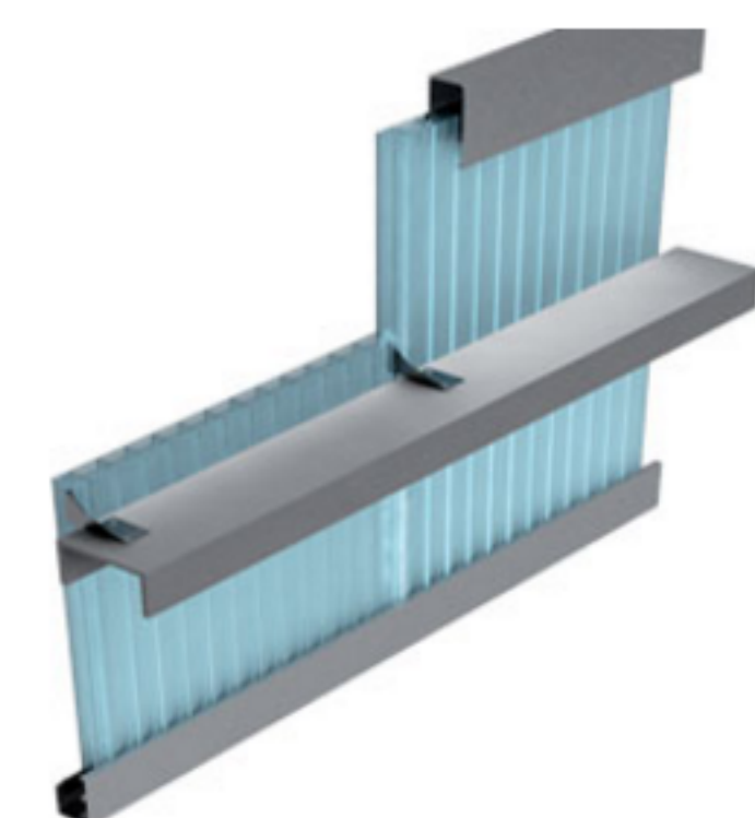
Positioning of anchor plates on section-breaker profile
