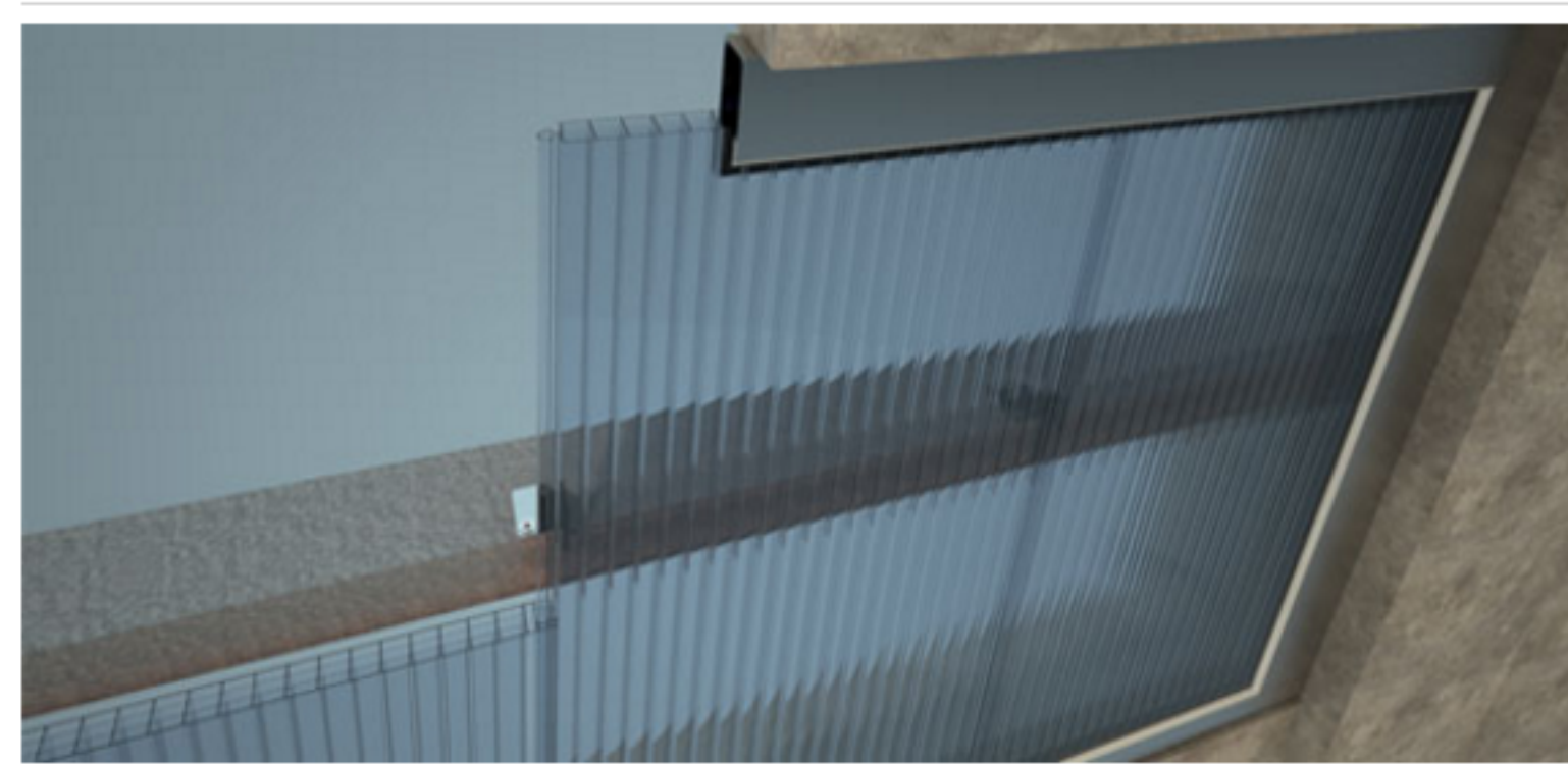
Construction of continuous transparent glazing, with section-breaker profile
